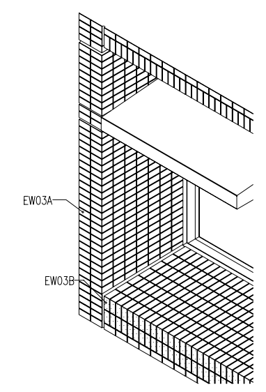
2 PILLAR & WINDOW TILE ISOMETRIC PROJECTION 柱子 & 窗戶瓷磚等角示意图 NO SCALE
